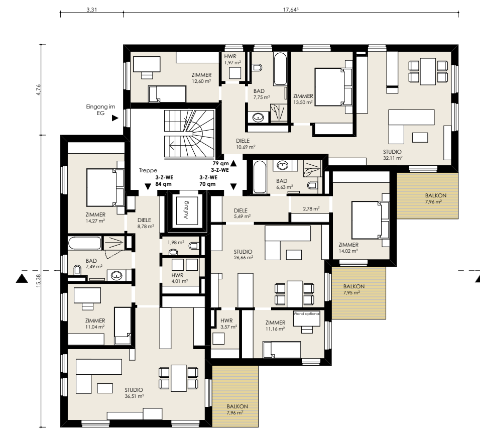
M 1_200 _ ERD- & OBERGESCHOSS_1
